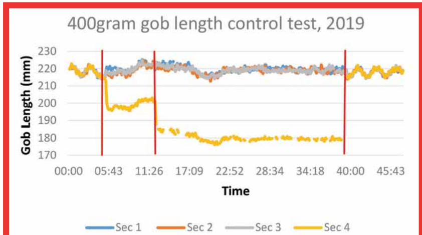
Fig 3. Section 4 gob length being shortened to 200mm and then to 180mm maintaining its weight.
